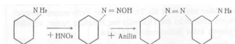
Aniline
